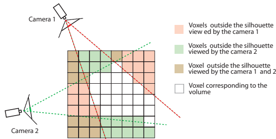
Figure 5: Principle of voxel carving.
